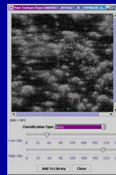
Extracted Texture
