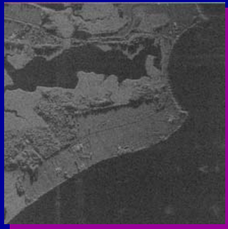
Raw Image
