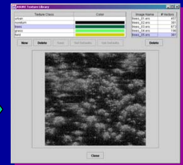
Texture Library
